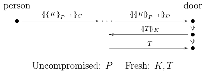
Figure 8.8: DoorSEP Weakness
